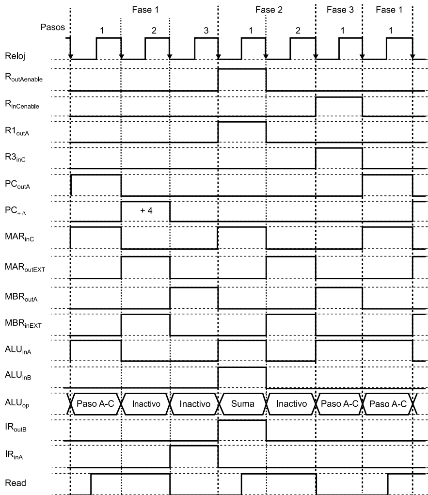
F1.P1: MAR \leftarrow PC, read
